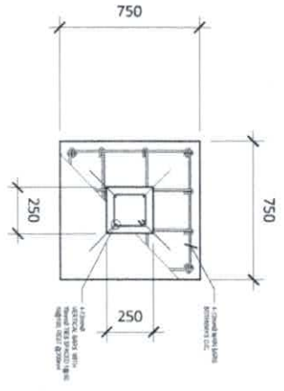
LIBRANG AIRPORT FOUNDATION AND COLUMN DETAIL SCALE
