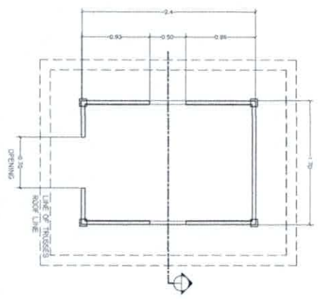
A PLAN SCALE 1:35 MTS
