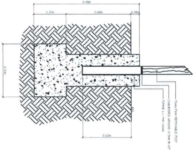
FOUNDATION PLAN SCALE 1:80
