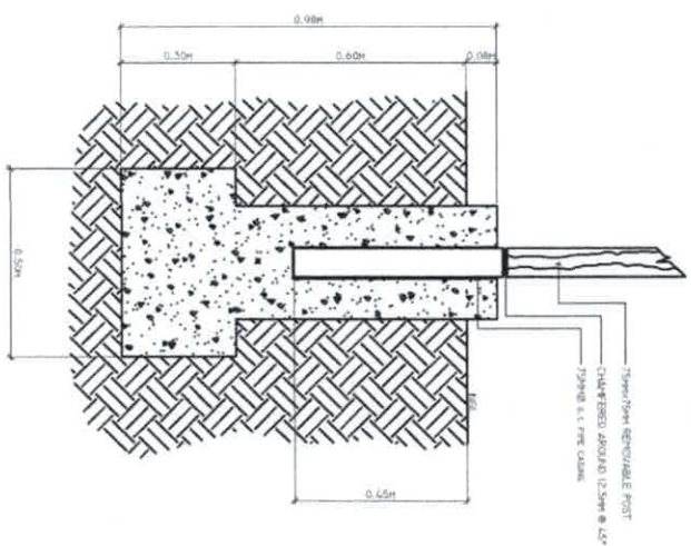
FOUNDATION PLAN SCALE 1:81
