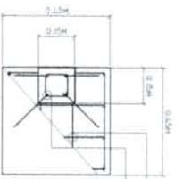
S-2 DETAIL OF C.I.F.L.
