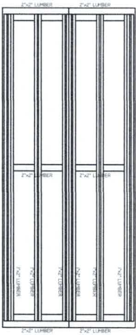
FRAMING PLAN SCALE 1:10 FT
