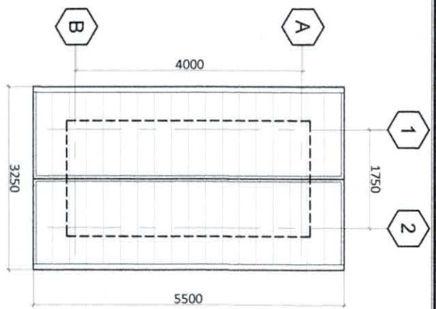
A ROOF PLAN SCALE 1:35 M.T.S
