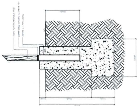
FOUNDATION PLAN SCALE 1:50
