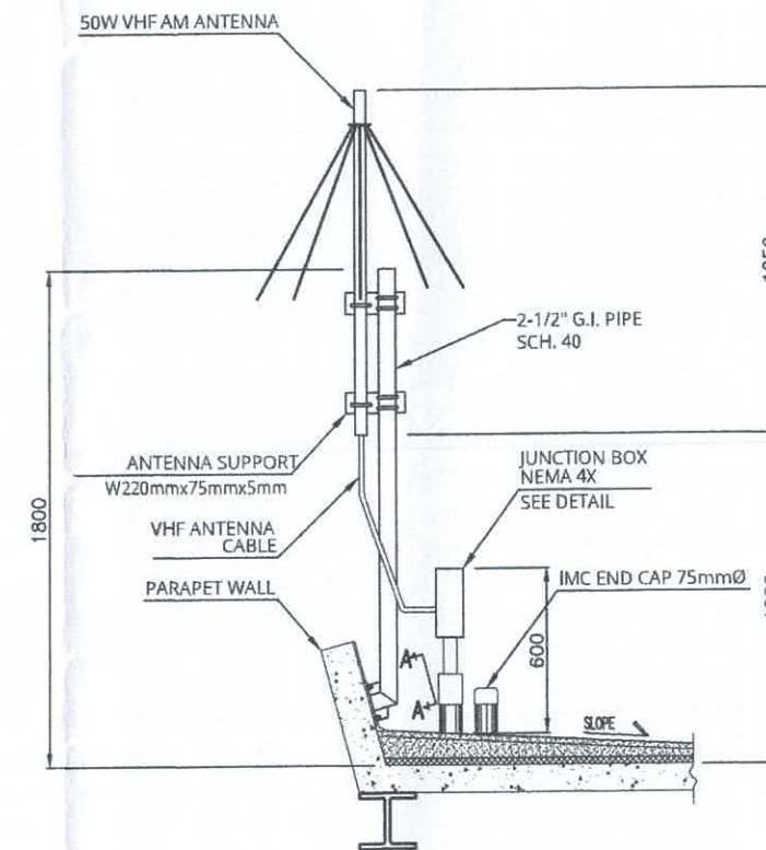
50W VHF AM TRANSMITTER ANTENNA VHF AM RECEIVER ANTENNA INSTALLATION DETAIL
