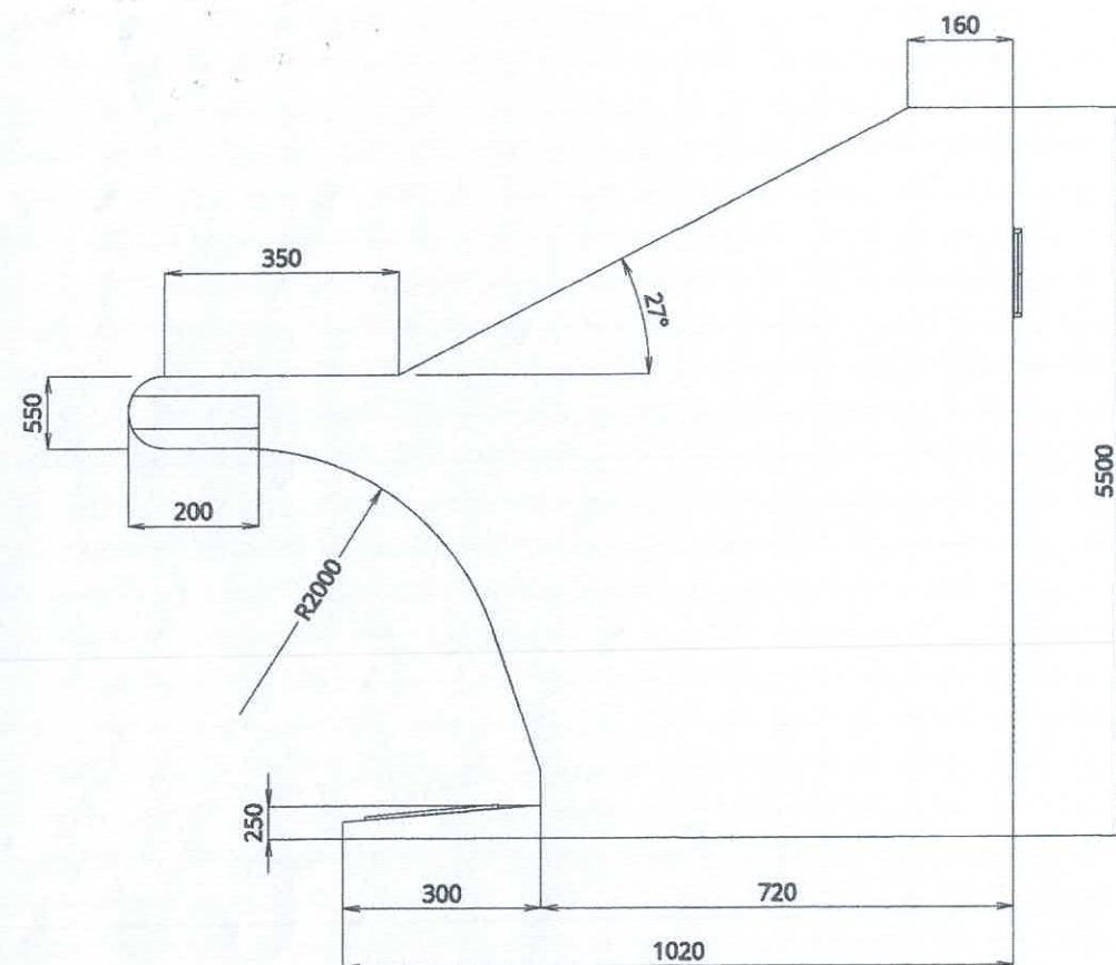
LEFT ELEVATION
