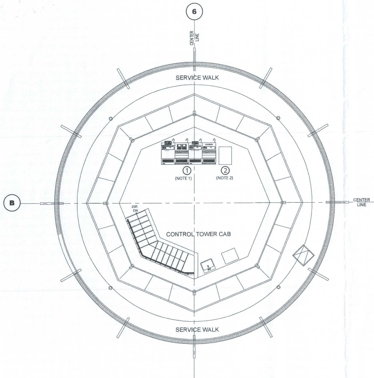
CAB ROOM EQUIPMENT LAYOUT SCALE NTS
